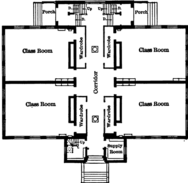
FIG. 16.—Sketch of building lighted from all sides and having four rooms on each floor. L. W. Robinson, architect.
